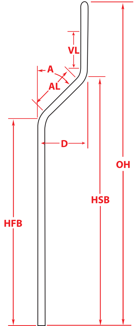
Right Side Double Bend
